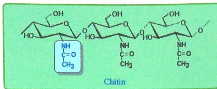
Figure 1: Chemical structure of chitin. (Bordenave, 2009)
