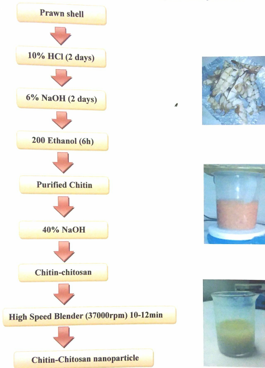
Figure 7: Preparation procedure of chitin-chitosan nanoparticle from prawn shell.
