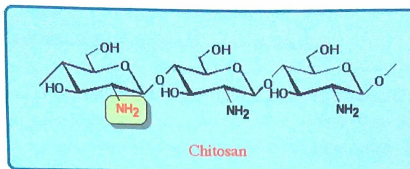
Figure 2: Chemical structure chitosan. (Bordenave, 2009)
